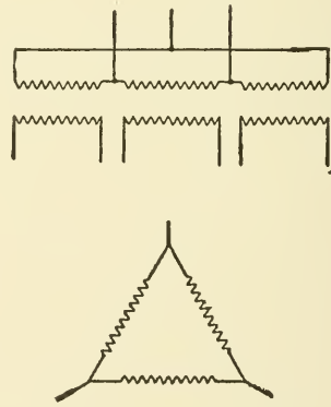
Fig. 30. Δ Connections for Transformers
